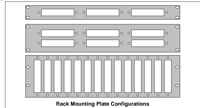
Rack Mounting Plate Configurations
